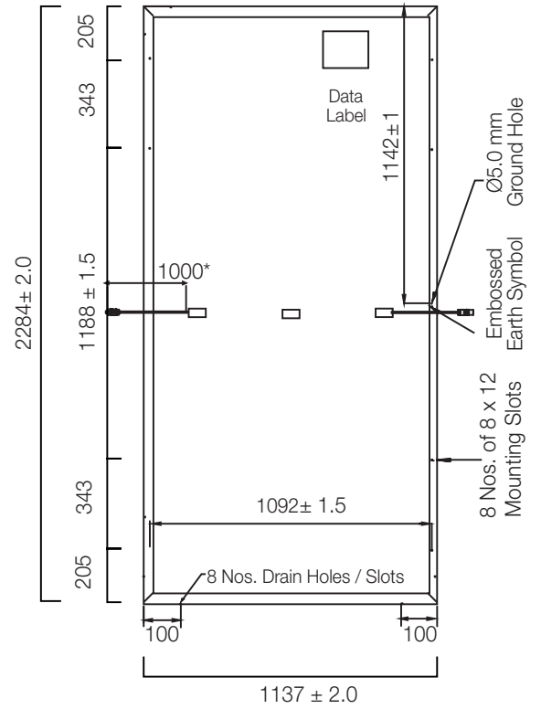
Module Dimension Diagram (mm)
